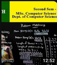
Pattern Matching
